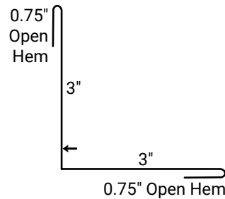
Inside Corner • 30IC
