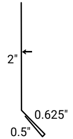
Lap Siding Starter • 30ST
