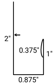
Invert J-Channel, color inside • 30JC
