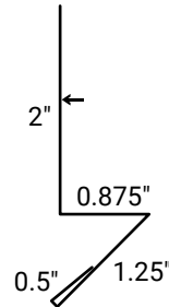
Rat Guard • 30RG
