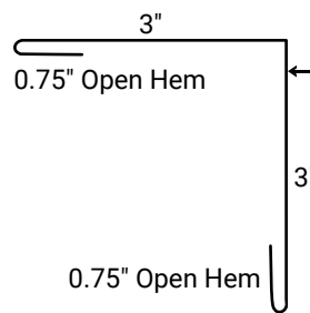
Outside Corner • 30OC
