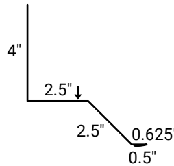
Step Sidewall
