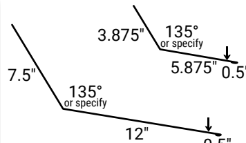
Endwall/Transition - SM or LG
