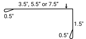
Fascia (1.5x3.5, 5.5 or 7.5)
