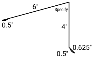
Denver High Side Peak
