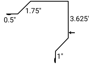
Outside Corner
