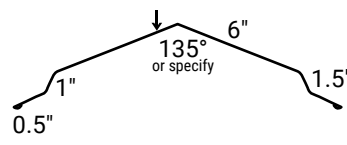
16" Ridge
