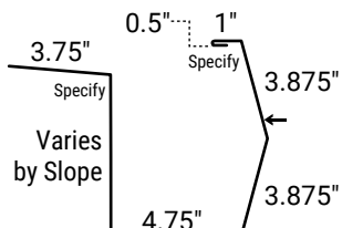
Sculptured Eave Gutter
