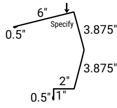
Sculptured High Side Peak
