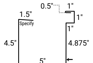
PBR Box Hang On Gutter
