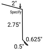
Denver Eave
