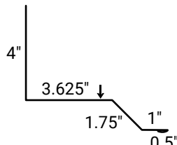
Sidewall
