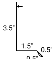
Drip Cap
