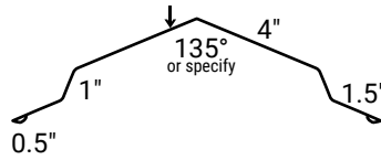
12" Ridge
