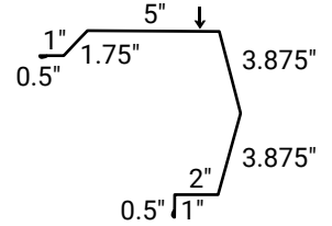
Sculptured Rake
