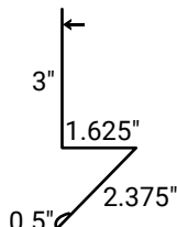
Rat Guard
