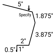
Sculptured Eave
