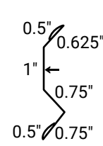
Counter Flashing
