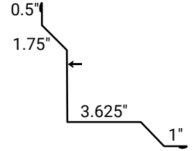
Inside Corner
