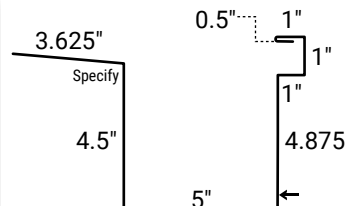
PBR Box Eave Gutter
