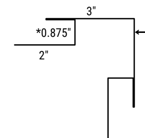
One Piece O/S Corner • 300CO *Alt 5/8" Gap • 300C058
