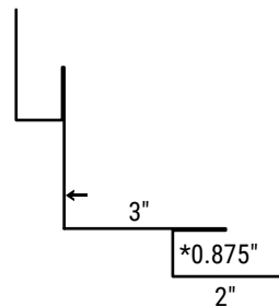
One Piece I/S Corner • 30ICO *Alt 5/8" Gap • 30IC058
