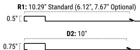
Craftsman Board & Batten • R1: 32, 31, 30, D2: 37
