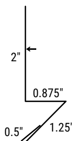
Rat Guard • 30RG
