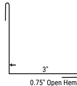
I/S Corner • 30IC
