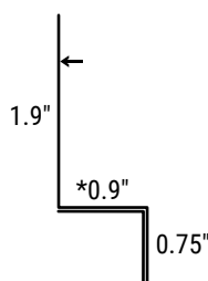
Doubleback Double Angle • 30DADB *Alt 5/8" Gap • 30DDADB58
