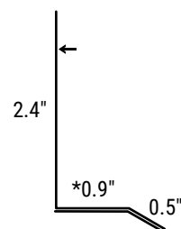
Doubleback Drip Cap • 30DCDB *Alt 5/8" Gap • 30DCDB58
