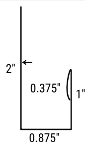
Invert J-Channel, color inside • 30JC
