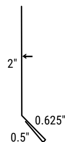
Lap Siding Starter • 30ST
