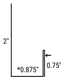
Doubleback J-Channel • 30JCDB *Alt 5/8" Gap • 30JCDB58
