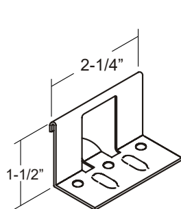
SL150 Clip 10 Standard clip, 20 ga Galvanized
