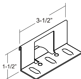
SL150 Clip 11 UL clip, 18 ga Galvanized
